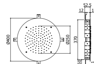
ZSOF 303CR LOS ANGELES Soffione ad incasso "Tondo" in metallo, anticalcare - Ø 400 mm "Round" concealed ceiling metal shower head, antiscalc system - Ø 400 mm
