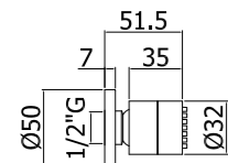
ZSOF 061CR Soffione tondo in metallo, anticalcare - Ø32 mm Round metal body jet, antiscald system Ø32 mm
