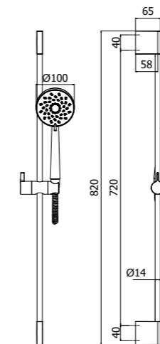
ZSAL 212CR LUNA TOP Saliscendi Luna Top con doccia (3 getti) in ABS Luna Top sliding rails with (3-spray functions) ABS hand-shower
