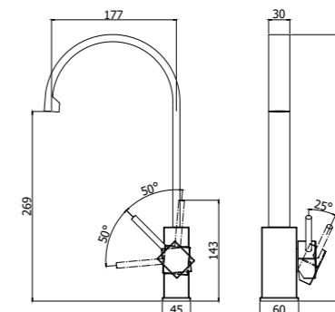
LEA 880CR Miscelatore lavello monoforo canna piatta orientabile One-hole sink mixer with rectangular swivelling spout
