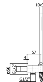
ZDUP 095CR QUADRO Set doccia incasso quadro con presa acqua incorporata Square concealed shower set with build-in water inlet
