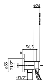
ZDUP 094CR TONDO Set doccia incasso tondo con presa acqua incorporata Round concealed shower set with build-in water inlet
