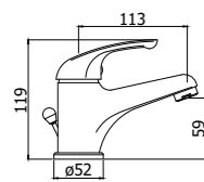
APM3 071-075CR Miscelatore lavabo con/senza scarico Wash basin mixer with/without pop up waste
