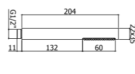
ZDOC 078CR BERRY Doccia Berry (monogetto) in metallo Berry (single-spray) metal hand-shower
