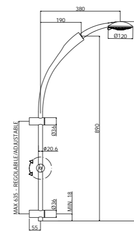
ZSAL 197CR TWIN Saliscendi Twin con doccia (4 getti) in ABS Twin sliding rails with (4-spray functions) ABS hand-shower
