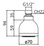
ZSOF 032CR OREGON Soffione "Oregon" in ABS, anticalcare Ø 70 mm "Oregon" ABS shower head, antiscald system - Ø 70 mm
