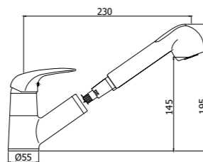
DU 183CR Miscelatore lavello con doccia estabile (2 getti) e canna tubo orientabile One-hole sink mixer with pull-out hand-shower (two-spray) and swivelling spout
