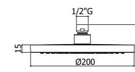
ZSOF 115CR PANDA Soffione "Panda" in ABS, anticalcare Ø 200 mm "Panda" ABS shower head, antiscalare system Ø 200 mm
