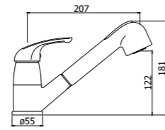
APM3 183CR Miscelatore lavello con doccia estraibile (2 getti) e canna tubo orientabile One-hole sink mixer with pull-out hand-shower (two-spray) and swivelling spout
