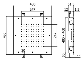
ZSOF 300CR NEW YORK Soffione ad incasso "Quadro" in metallo, anticalcare - 430x430 mm "Square" concealed ceiling metal shower head, antiscalc system - 430x430 mm
