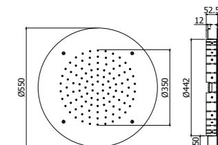
ZSOF 304CR LAS VEGAS Soffione ad incasso "Tondo" in metallo, anticalcare - Ø 550 mm "Round" concealed ceiling metal shower head, antiscalc system - Ø 550 mm
