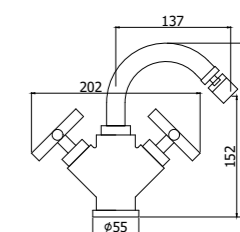
QTV 138-137CR Monoforo bidet con/senza scarico One-hole bidet mixer with/without pop up waste
