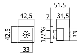
ZSOF 062CR Soffione quadro in metallo, anticalcare - 33x33 mm Square metal body jet, antiscald system - 33x33 mm
