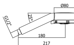
ZDOC 070CR MAJORCA Doccia Majorca (3 getti) in ABS Ø80 mm Majorca (3-spray functions) ABS hand-shower Ø80 mm
