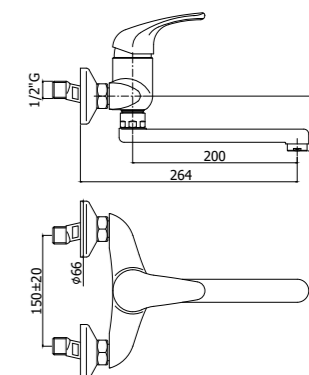
ND 161CR Miscelatore lavello a muro con canna tubo orientabile Wall sink mixer with swivelling tube spout
