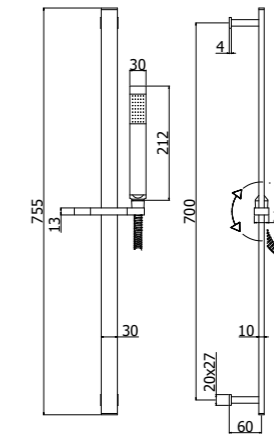
ZSAL 145CRAG CITY Saliscendi City con doccia (monogetto) in metallo City sliding rails with (single-spray) metal hand-shower
