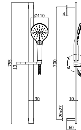
ZSAL 147CRAG CITY SOFIA Saliscendi City Sofia con doccia (2 getti) in ABS City Sofia sliding rails with (2-spray functions) ABS hand-shower
