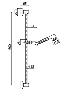
ZSAL 010CR KLIPPER Saliscendi Klipper con doccia (monogetto) in metallo Klipper sliding rails with (single- spray) metal hand-shower
