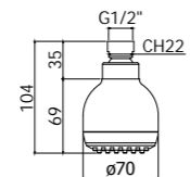
ZSOF 031CR ALABAMA Soffione "Alabama" in ABS, anticalcare Ø 70 mm "Alabama" ABS shower head, antiscald system - Ø 70 mm
