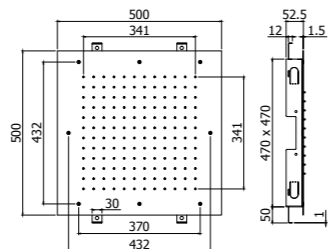
ZSOF 301CR BOSTON Soffione ad incasso "Quadro" in metallo, anticalcare - 500x500 mm "Square" concealed ceiling metal shower head, antiscalc system - 500x500 mm
